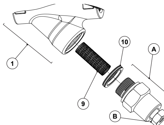
Fig. 6: BDV blowdown valve.
