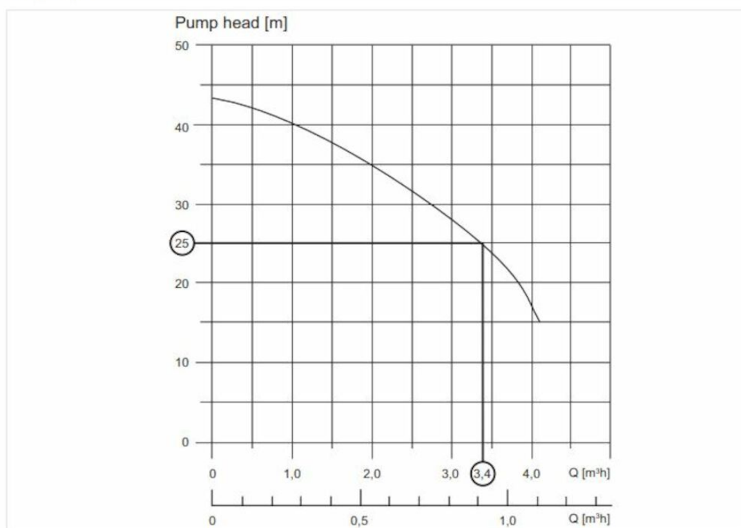
Pump Output
