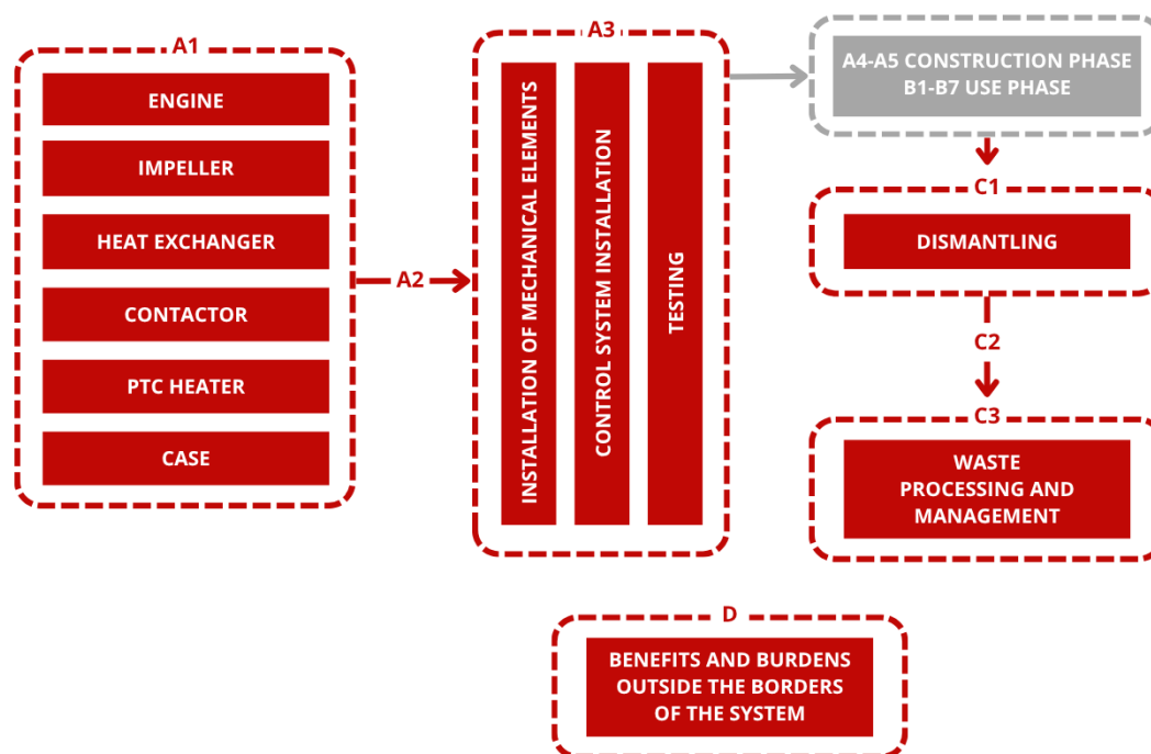
Figure 5.1: System boundaries for the environmental characteristics of Guard air curtains
