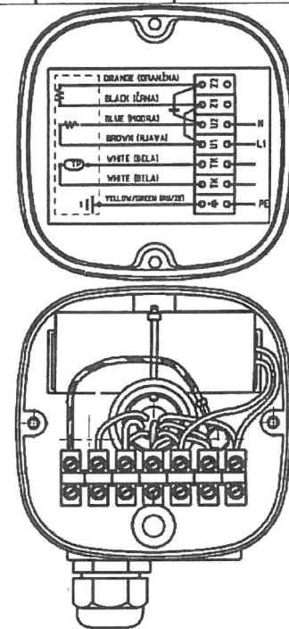
CONNECTION DIAGRAM
