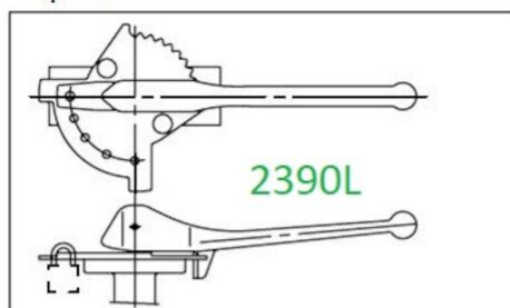
FIG. 1: LEVER + PADLOCK FACILITY
