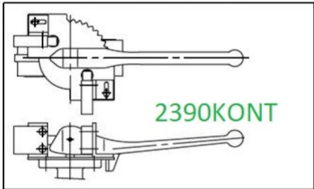
FIG. 2: LEVER + SWITCHES
