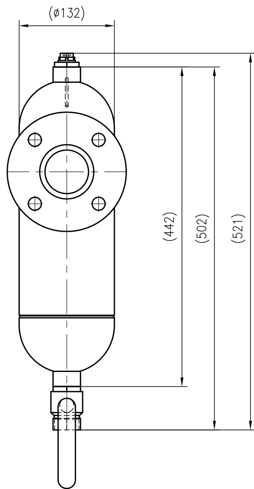
Side view
