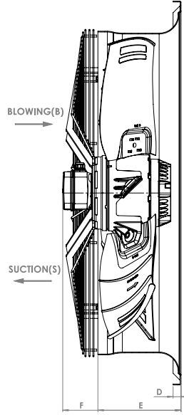
Dimensions [mm]
