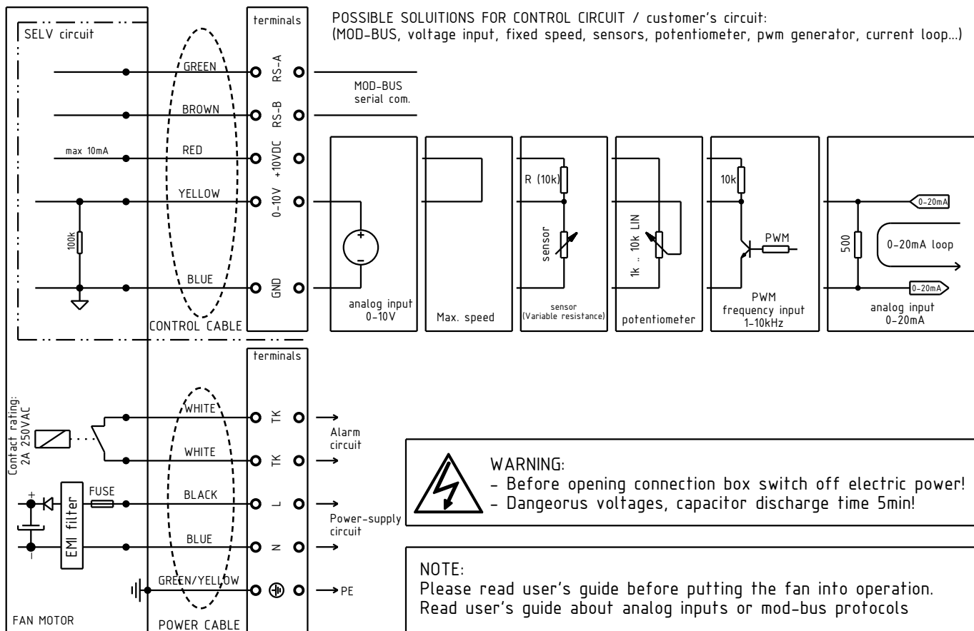
Connecting diagram 0302-0-0006
