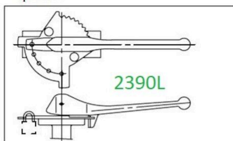
FIG. 1: LEVER + PADLOCK FACILITY
