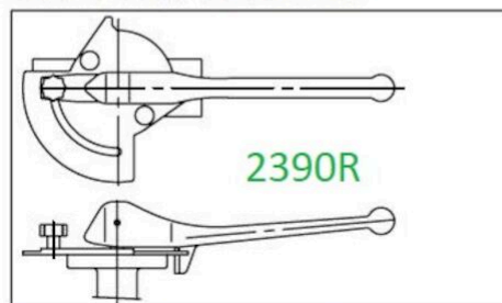
FIG. 3: LEVER FOR REGULATING
